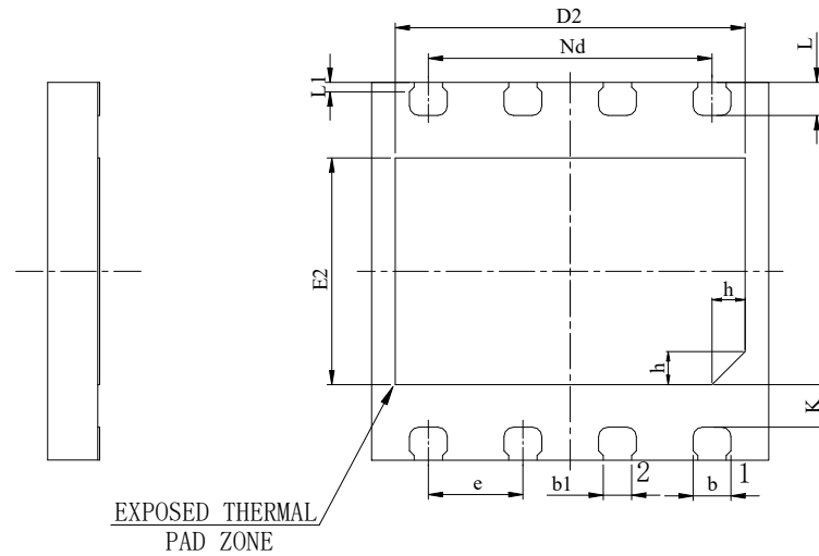
BOTTOM VIEW
