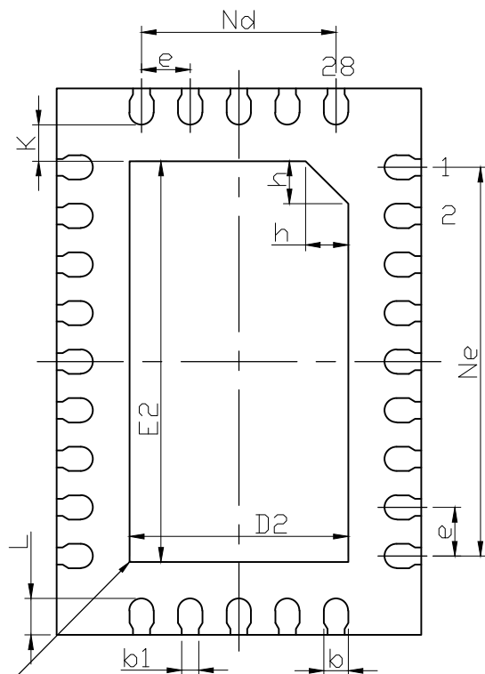
BOTTOM VIEW
