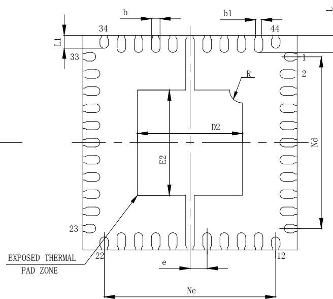
BOTTOM VIEW
