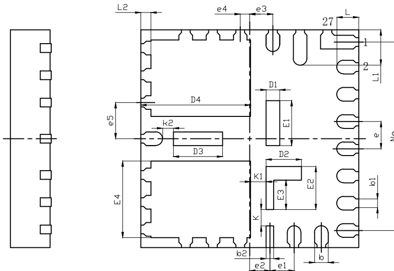
BOTTOM VIEW
