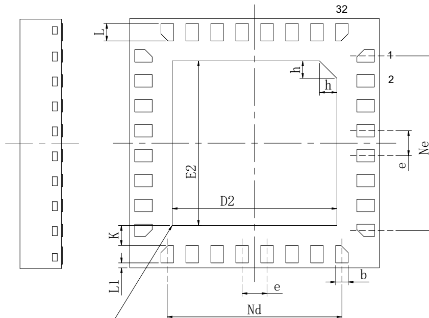
BOTTOM VIEW
