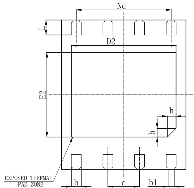
BOTTOM VIEW
