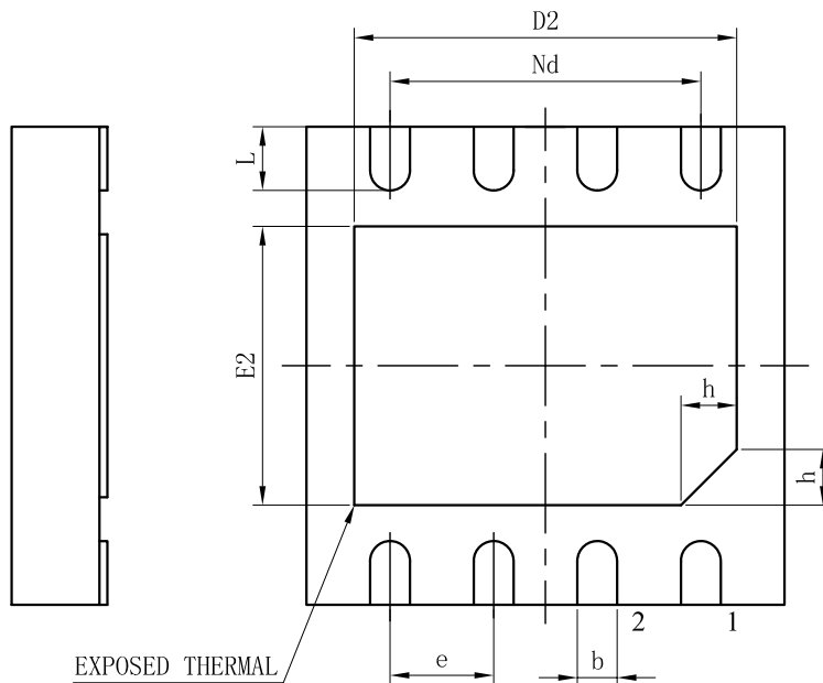
BOTTOM VIEW
